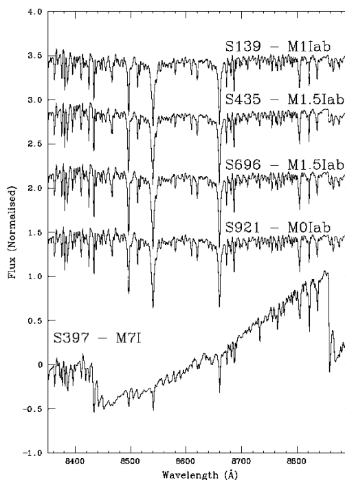
Figure 3: Spectra of the five red supergiants in NGC 7419, in the region of the Ca II triplet.
